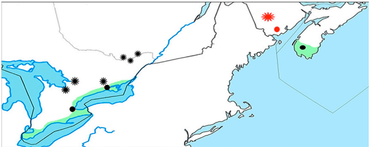
Map 1. Merycomia whitneyi : Previous records ● new record ● Hybomitra cincta : Previous records * new record *
